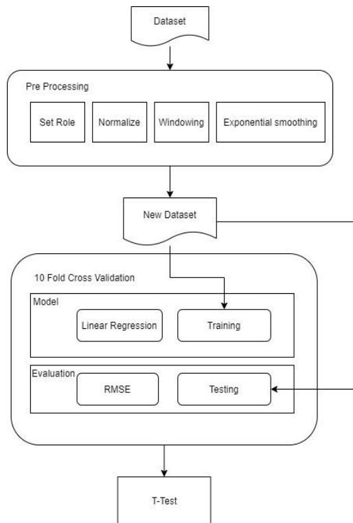
Figure 1. Proposed Method
